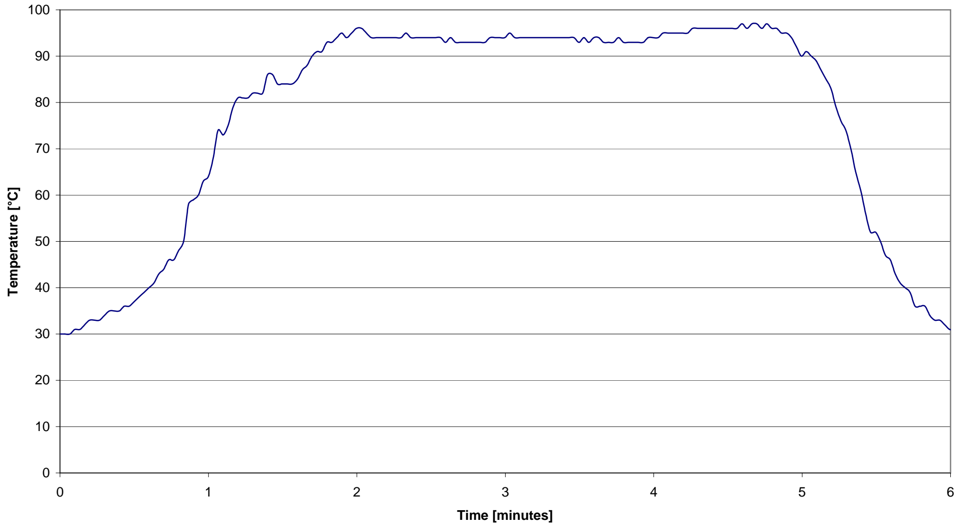
PD977 Cure Profile [90°C for 3 minutes]
